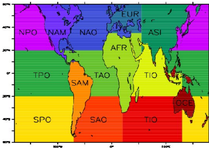
Fig. 1. Definition of the 14 different regions (see Table 1 for acronyms).
