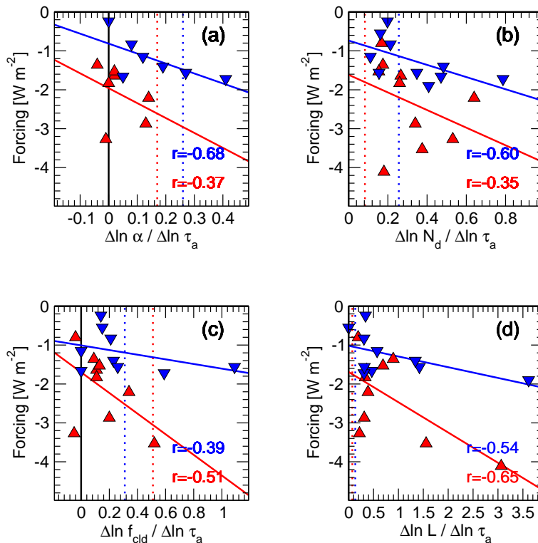
Fig. 7. Influence of the relationships between \tau_a and (a) \alpha , (b) N_d , (c) f_{\text{clid}} and (d) L on the total short-wave aerosol forcing over land (red) and oceans (blue), for the up to ten different GCMs (the data are listed in Table 2). The plain lines show the linear regression between the slopes and the forcing, and the dashed vertical lines show the slopes inferred from the MODIS Terra (MODIS-CERES-Terra for \alpha ) satellite retrievals.
