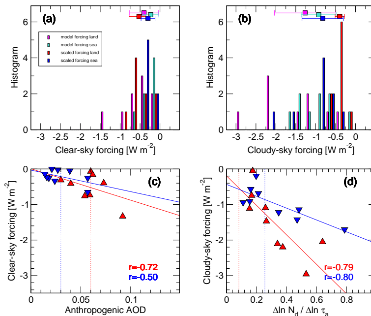
Fig. 8. Forcing estimates. (a) Clear-sky short-wave aerosol forcing histograms (in bins of width 0.25 \text{ W m}^{-2} ) for the original model estimates as mean values over land (magenta) and oceans (turquoise), and rescaled using the relationship clear sky forcing – anthropogenic \tau_a shown in (c) applying the satellite-based estimate for anthropogenic \tau_a by Bellouin et al. (2005) over oceans (dashed blue line) and the model-median anthropogenic \tau_a over land (dashed red line) over land (red) and oceans (blue). (b) Cloudy-sky short-wave aerosol forcing histograms ( 0.25 \text{ W m}^{-2} bin width), with rescaled forcing estimate using the cloudy sky forcing vs. N_d - \tau_a -regression-slope relationship shown in (d) applying the MODIS Terra-derived N_d - \tau_a slope estimate. The median forcing values and standard deviation are shown on the top of (a) and (b) (see listing in Table 4). Clear and cloudy sky forcings are scaled by the clear and cloudy fraction as in Table 3.
