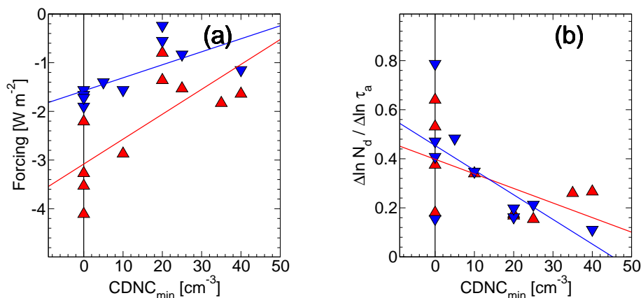
Fig. 6. The imposed lower limit on N_d vs. (a) total short-wave aerosol radiative forcing and (b) relationship N_d - \tau_a over land (red) and ocean (blue). ECHAM5 uses a lower limit of 40 cm^{-3} ; Hadley, 35 cm^{-3} over land and 5 cm^{-3} over ocean; SPRINTARS, 25 cm^{-3} ; GISS and LMDZ-INCA, 20 cm^{-3} ; CAM-Umich, 10 cm^{-3} , and CAM-NCAR, CAM-Oslo, CAM-PNNL, and GFDL, no lower limit.
